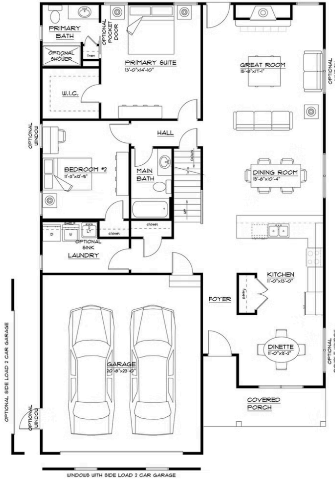
FIRST FLOOR PLAN THE "ANGELINA 225" 2/5/2025 LIVING AREA: 1550 S.F. OVERALL DIMENSIONS: 31'-4" x 59'-0"
