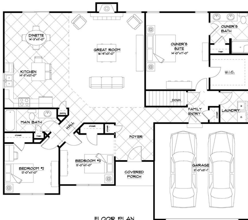
FLOOR PLAN THE "AVERY 22A" 3/1/2022 LIVING AREA: 1812 S.F. OVERALL DIMENSIONS: 55'-0" x 41'-4"
