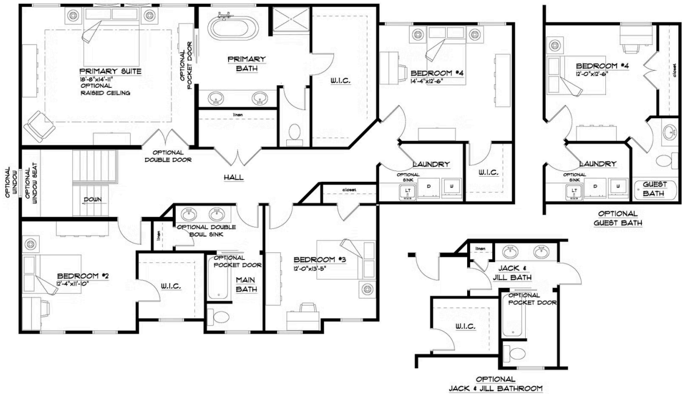
SECOND FLOOR PLAN THE "NEWPORT 24A" 4/5/2024 LIVING AREA: 1662 S.F.
