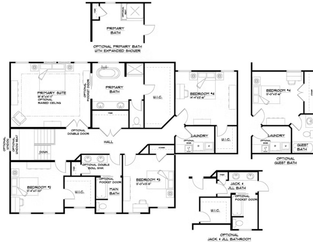
SECOND FLOOR PLAN THE "NEWPORT 24A" 4/5/2024 LIVING AREA: 1662 S.F.
