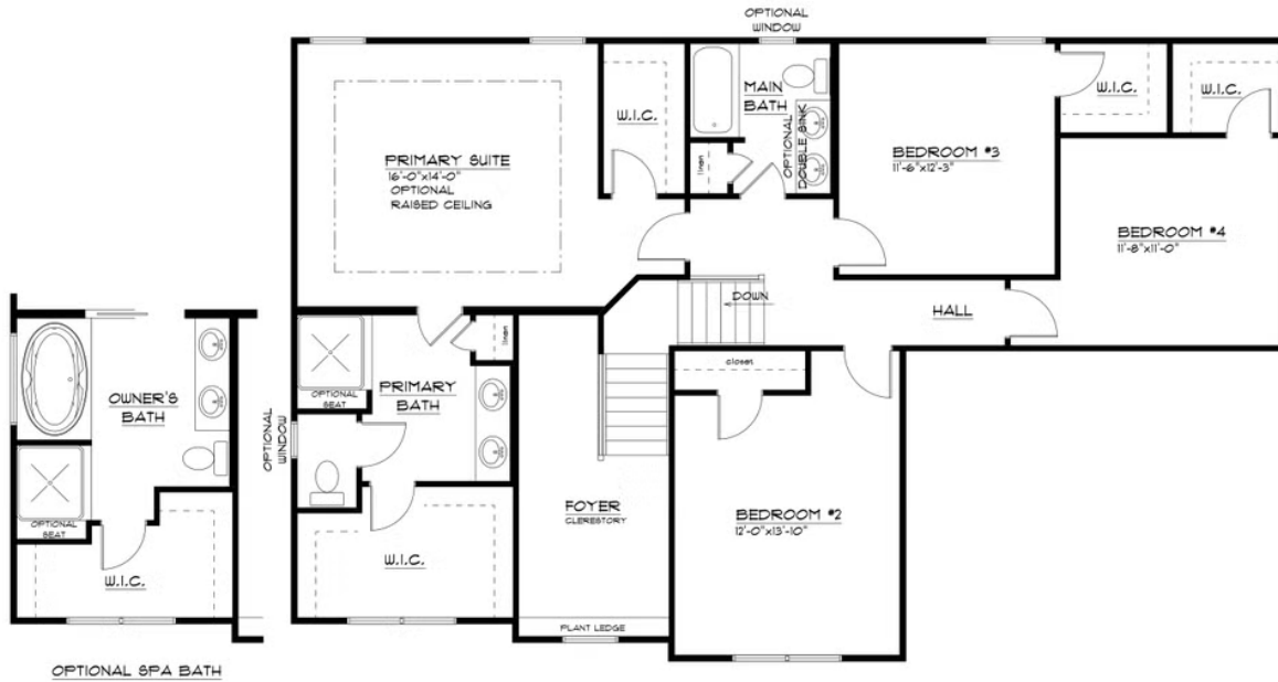
SECOND FLOOR PLAN THE "HAWTHORNE 22A" 1/5/2023 LIVING AREA: 1265 S.F. CLERESTORY 133 S.F. TOTAL AREA 1398 S.F.
