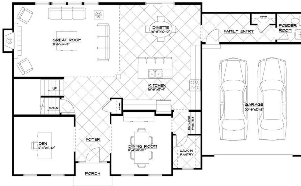
FIRST FLOOR PLAN THE "NEWPORT 22A" 3/9/2022 LIVING AREA: 1502 S.F.
