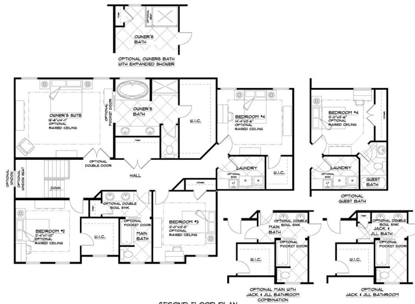
SECOND FLOOR PLAN THE 'NEWPORT 20A' 6/3/201 LIVING AREA: 1662 S.F.
